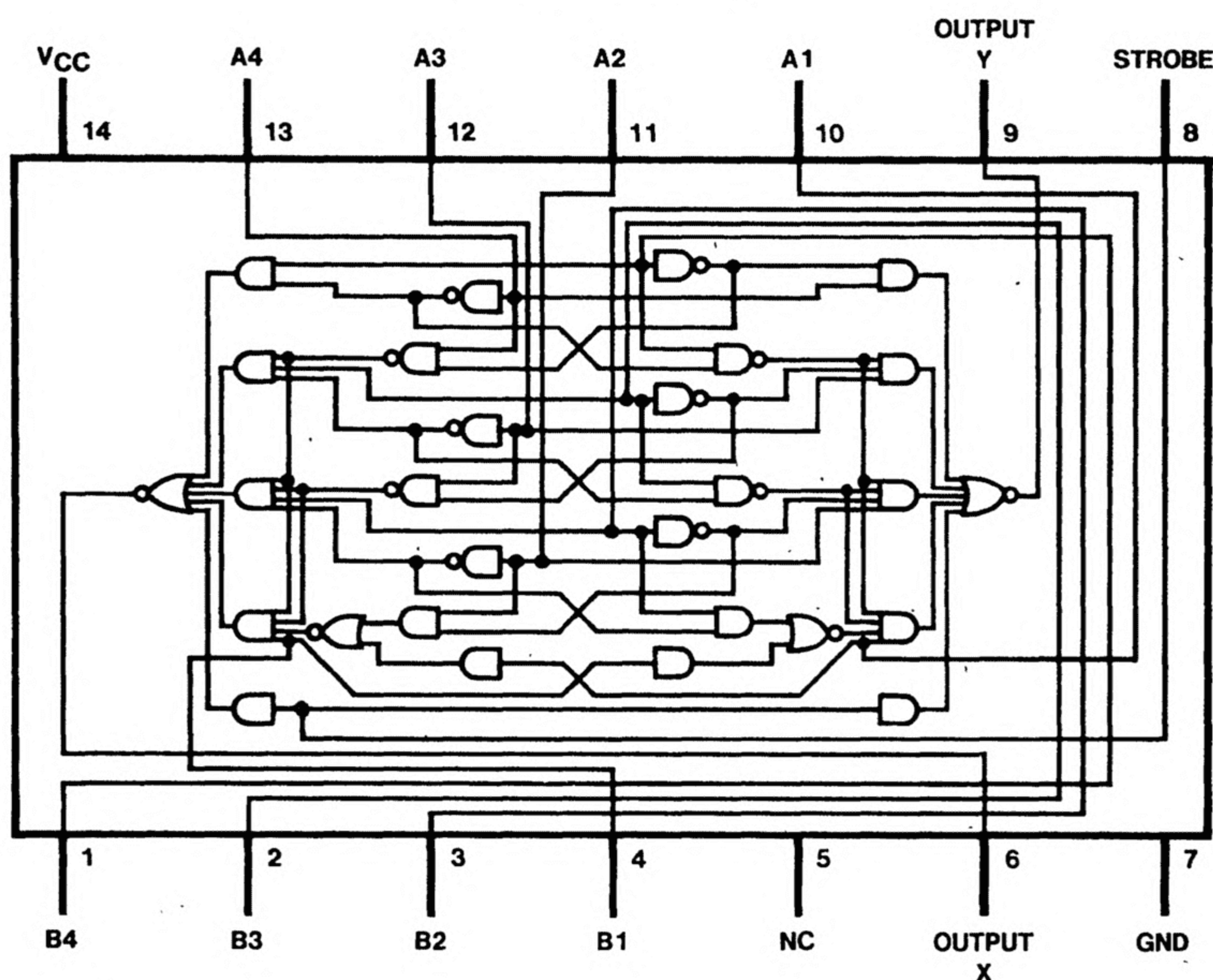
Dual-In-Line Package
