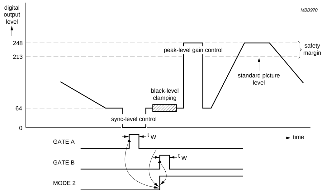
Fig.5 Control mode 2.
