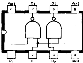
C54 DM8305N Dual MOS memory driver
