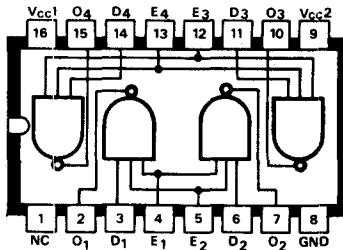
C53 DM8304N Quad MOS memory driver
