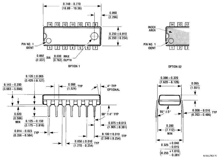
14-Lead Molded Dual-In-Line Package (N) Order Number DM7402N NS Package Number N14A
